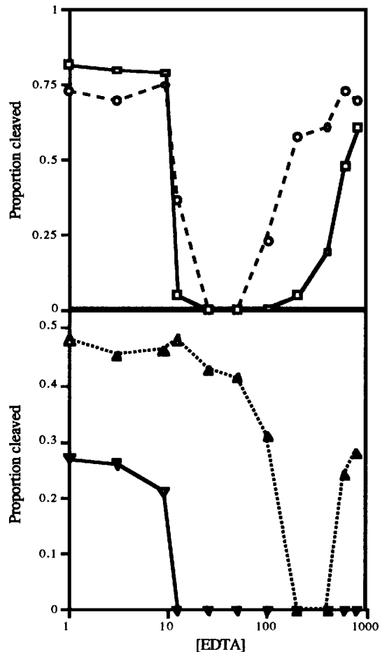
Fig. 4. Na 3 EDTA titrations demonstrate that magnesium-dependent ribozyme-catalyzed RNA cleavage reactions of the HH 16.1 (□), Hairpin (○) and VS (△) ribozymes but not the HDV ribozyme (▽) are quenched by EDTA and stimulated by monovalent cations (Murray et al. 1998b).
