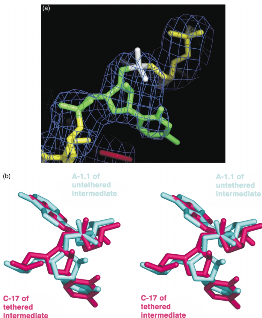
Figure 3. A trapped conformational change. (a) The cleavage site conformational change that aligns the attacking nucleophile of C17 (in green) with the scissile phosphate (in white). About 25^\circ of further rotation of the base and ribose of C17, or a concomitant sugar pucker, will complete the alignment while pushing the 2' oxygen atom to within bonding distance of the scissile phosphorus atom, presumably in a concerted manner. The \sigma -A weighted 2F_o - F_c electron density map (blue mesh) is contoured above 1.5 times the r.m.s.d. of the map. (b) A comparison of the conformationally changed structure having the Stem I-Stem II tether reported here (magenta) to the previous “late” intermediate structure (cyan) that lacks the tether, showing an overall similarity but suggesting that the new structure reported here is somewhat nearer to the pentacoordinate transition-state structure.
