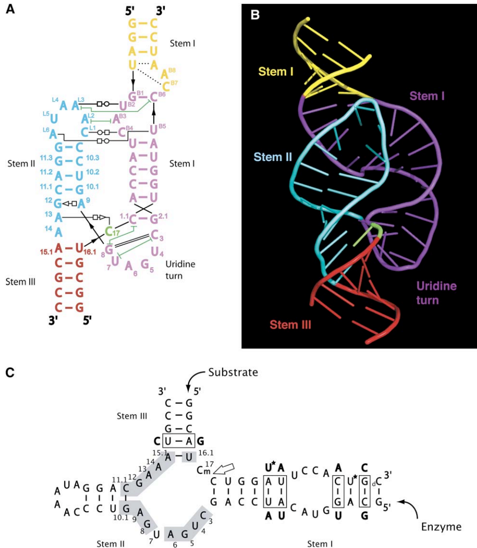
Figure 1. The Sequence and the Structure
