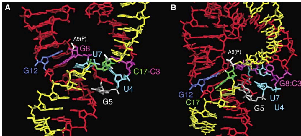
Figure 3. Side-by-Side Comparison of the Minimal and Full-Length Hammerhead Ribozyme Structures
