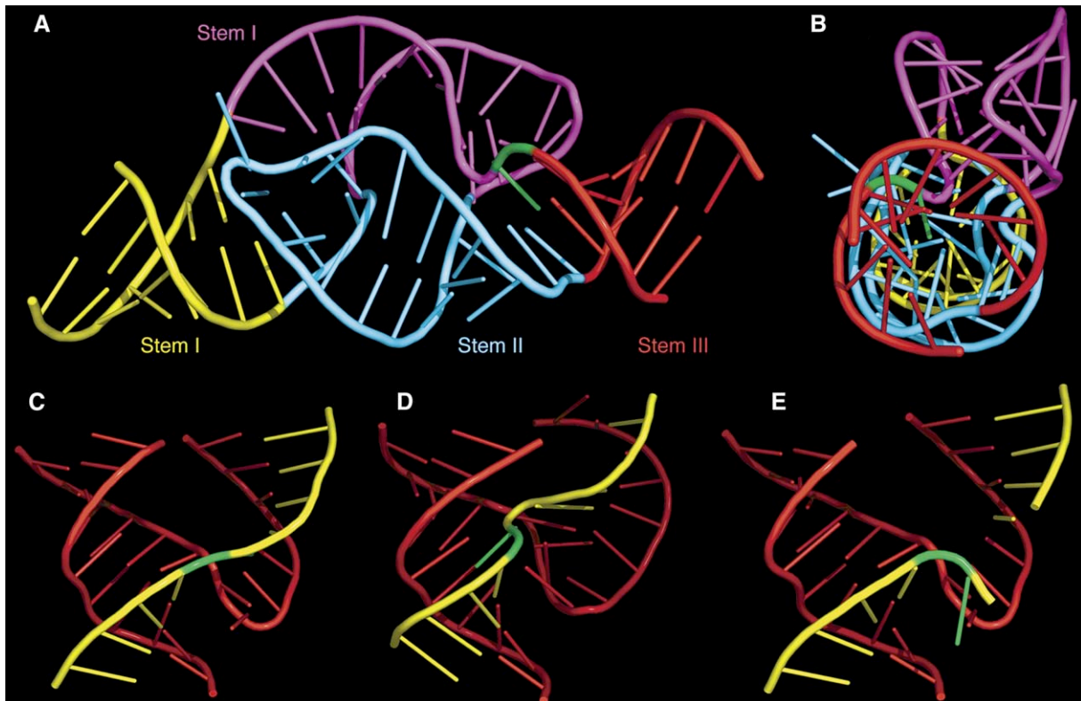
Figure 5. Aspects of the Full-Length Hammerhead Ribozyme Fold
